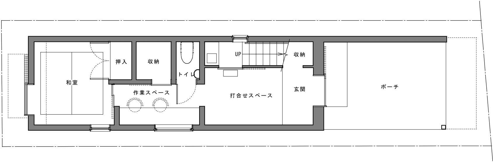
1F PLAN
